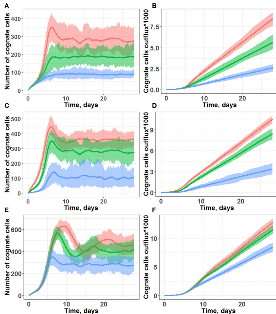
FIGURE 3 | Simulations of cognate T cell numbers in the LN T-zone (A,C,E) and their cumulative outflux through efferent lymphatics (B,D,F). (A,B) Simulations under scenarios of different chemotaxis probabilities. Multiple chemotaxis strength values were tested: 1/8 (blue line), 1/4 (green line), and 1/3 (red line). The maximal number of divisions was set at 10, and the cognate frequency was set at 1/100. (C,D) Simulations under scenarios of different cognate clone frequencies. Multiple cognate frequency values were tested: 1/50 (red line), 1/100 (green line), and 1/500 (blue line). The maximal number of divisions was set at 10, and chemotaxis strength was set at 1/3. (E,F) Simulations under scenarios of different maximal numbers of divisions: 10 (blue line), 15 (green line), and 20 divisions (red line). The cognate frequency was set at 1/100, and chemotaxis strength was set at 1/3. All plots are based on measures from 45 simulations lasting 28 days each. Lines represent median values; shaded areas represent 90% PI.
